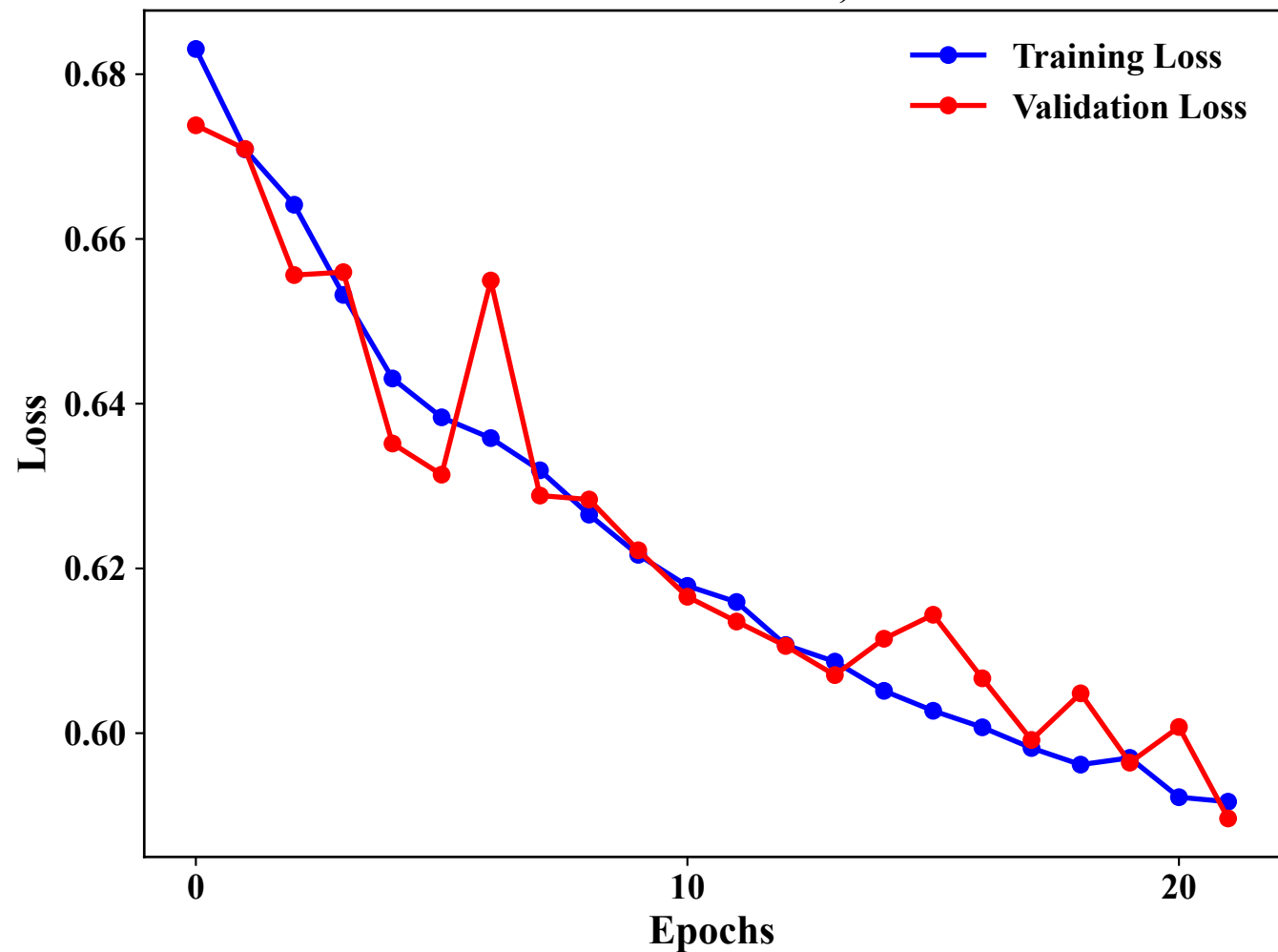
Loss Curves: Seed 32, Rank 1
